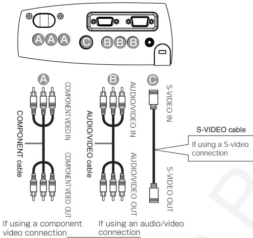
DVD player
